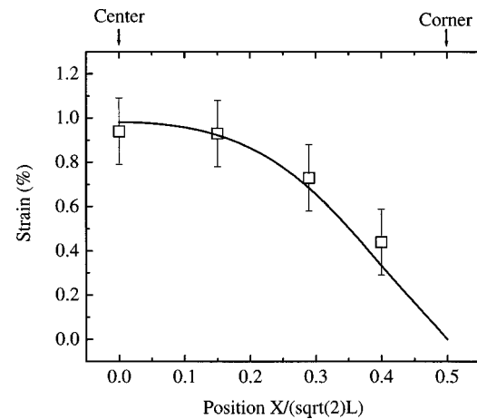
FIG. 4. Strain distribution along the diagonal of a 60\ \mu\text{m} \times 60\ \mu\text{m} island after a 17 min annealing at 790\ ^\circ\text{C} . Open squares are experimental data and the solid line is the fitting based on the 2D lateral expansion theory (see Ref. 13). The surface roughness rms of the island center is about 1 nm due to buckling, whose contribution to strain relaxation is negligible. L denotes island edge length, which is 60\ \mu\text{m} in this case.
