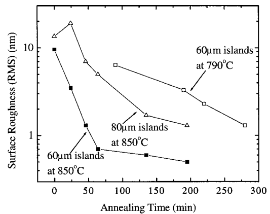
FIG. 11. Surface roughness as a function of annealing time at island center for 60 and 80 \mu\text{m} islands at 790 and 850 °C for \text{Si}_{0.70}\text{Ge}_{0.30} thickness of 30 nm. Samples annealed at 850 °C initially have a buckled \text{Si}_{0.70}\text{Ge}_{0.30} surface because they first went through an annealing of 35 min at 800 °C.
