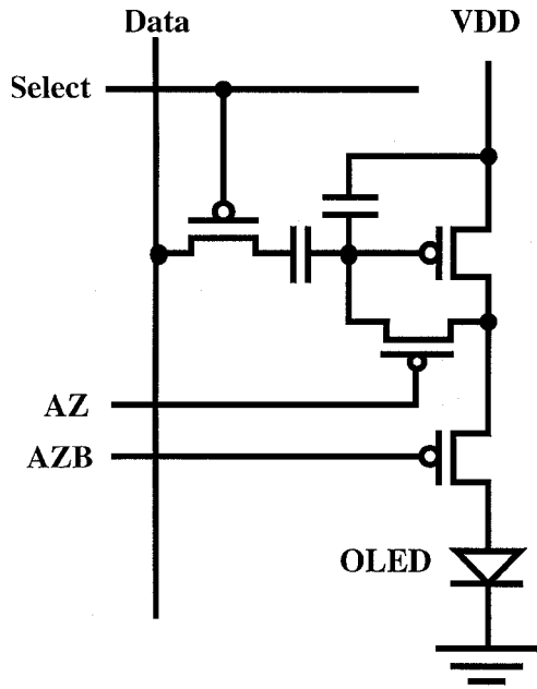
Fig. 3. Schematic of Four-Transistor AMOLED Pixel with Autozero.
