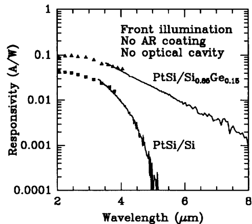
Figure 7: Comparison of measured external responsivities of \text{PtSi}/\text{Si}_{0.85}\text{Ge}_{0.15} and \text{PtSi}/\text{Si} infrared detectors. Points represent data obtained with a calibrated infrared monochromator (40K), while lines are scaled results from FTIR measurements.
