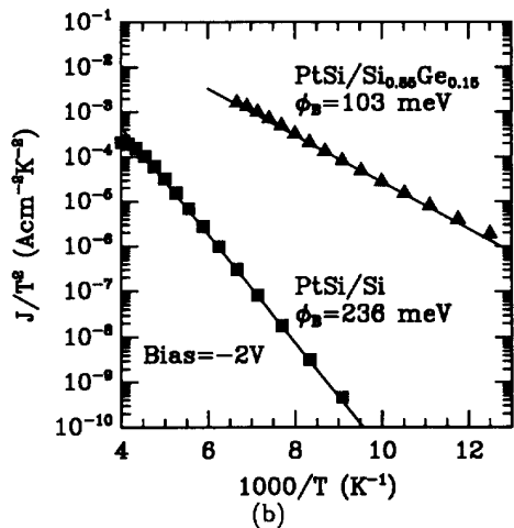
Figure 5: Temperature dependent dark current densities of (a) \text{Pd}_2\text{Si}/\text{Si}_{1-x}\text{Ge}_x and (b) \text{PtSi}/\text{Si}_{1-x}\text{Ge}_x detectors at 2V reverse bias. Schottky-barrier heights obtained from these I-T data (except for the \text{PtSi}/\text{Si}_{0.85}\text{Ge}_{0.15} device) agree with those obtained from optical measurements within 15 meV.
