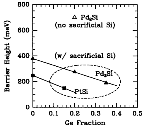
Figure 6: Schottky-barrier heights as functions of Ge fraction of both \text{Pd}_2\text{Si}/\text{Si}_{1-x}\text{Ge}_x and \text{PtSi}/\text{Si}_{1-x}\text{Ge}_x detectors obtained from photo-response measurements.
