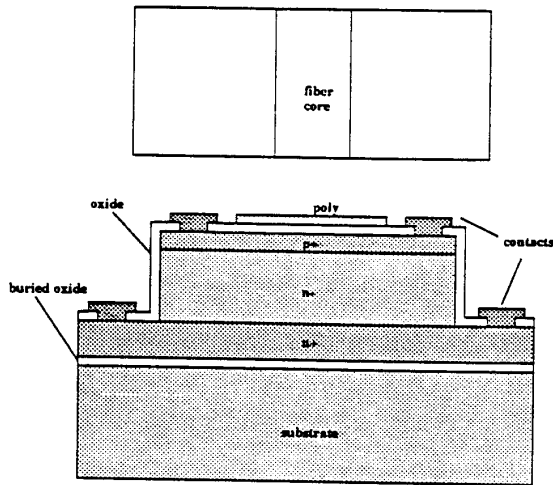
Figure 1. Schematic diagram of the device structure
