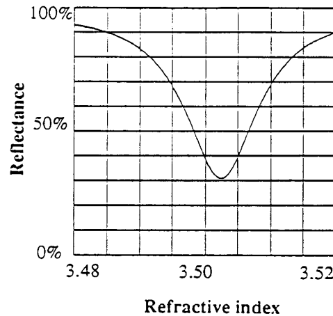
Figure 2. Calculated reflectance of device structure as a function of silicon refractive index.
